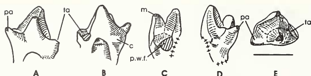
TEXT-FIG. 2. Dorsetodon haysoni gen. et sp. nov.; holotype DORCM GS 433; lower right molar. A, lingual view; B, labial view; C, posterior view; D, anterior view; E, occlusal view. Key: m, metaconid; pa, paraconid; pr, protoconid; p.w.f., posterior wear facet; ta, talonid. Hatching, wear; cross-hatching or crosses, broken areas or edges. Scale bar represents 0.5 mm.
